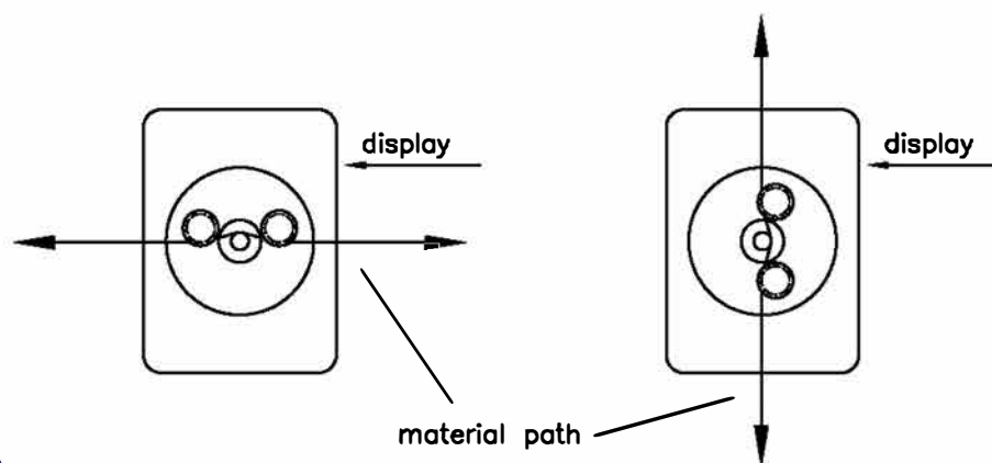
view A
