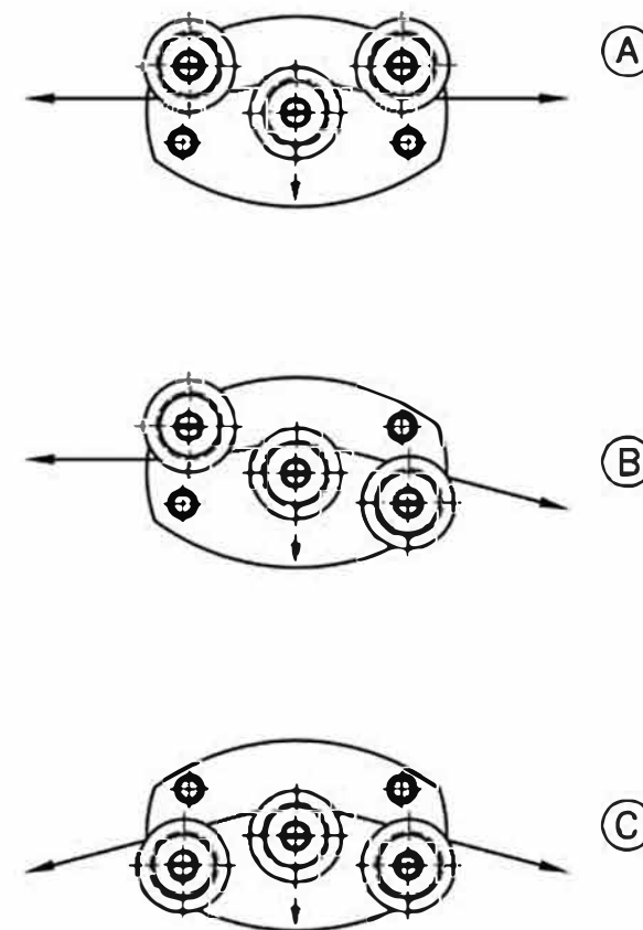
possible material path and corresponding guide roller position
