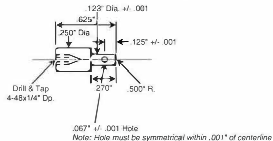
Swivel Connector Top
