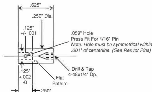
DESCRIPTION: SWIVEL CONNECTOR PART NO: DETAIL MTG-02
