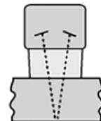
Dual Element Transducer in Echo-Echo mode
