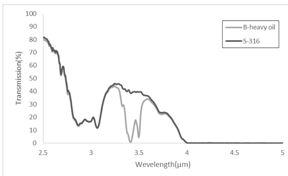
Fig. 84 Infrared absorption spectrums of solvent S-316 and oil
