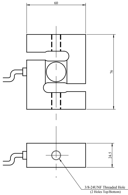
DPU-220 Dimensions in mm
